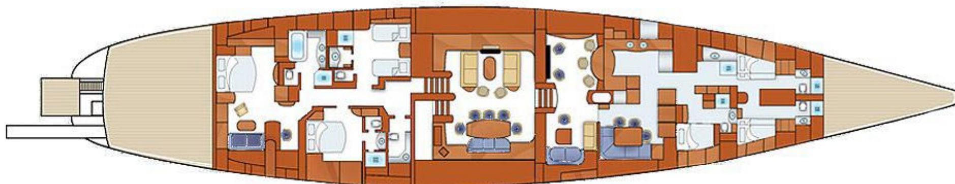
LOWER DECK
